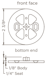
INSIDE/JAMB MOUNT: DRIVE SIDE SHA-B2XX
