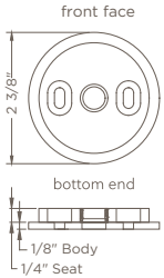
INSIDE/JAMB MOUNT: IDLER SIDE SHA-B1XX
