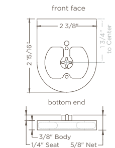
FLOATING/OUTSIDE MOUNT MANUAL: DRIVE SIDE SHA-B4MANUALXX
