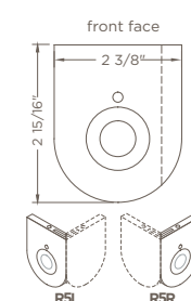
90° ANGLE/CORNER MOUNT SHA-B7XX & SHA-B8XX
