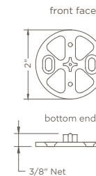
INSIDE/JAMB MOUNT MINI: DRIVE SIDE SHA-B2MINXX
