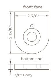
SHADE COUPLER SHA-B5XX
