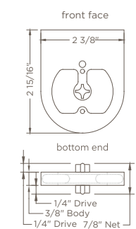
DUAL MOTOR MOUNT & WIDE SHADE COUPLER SHA-B6XX & SHA-B5WXX
