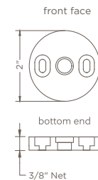
INSIDE/JAMB MOUNT MINI: IDLER SIDE SHA-B1MINXX
